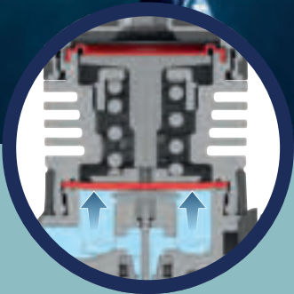
Auto-Balanced (also known as Over-Balanced)
